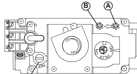
PILOT SCREW
